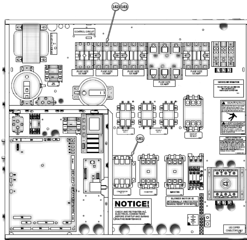
EP COMPRESSOR CIRCUIT FUSED
