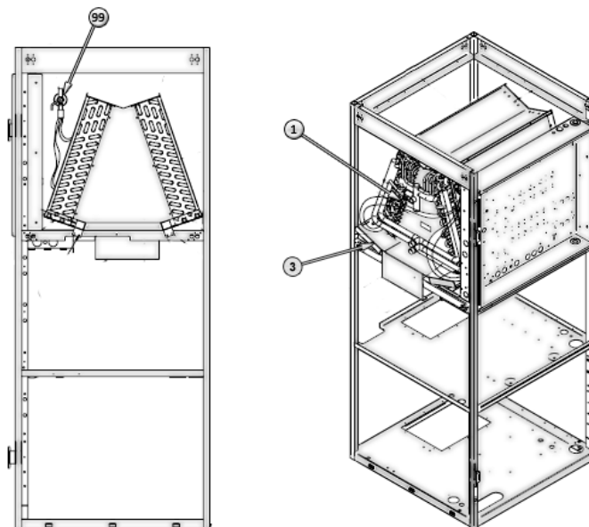
COIL OPTION 5T DOWNFLOW RIFLED
