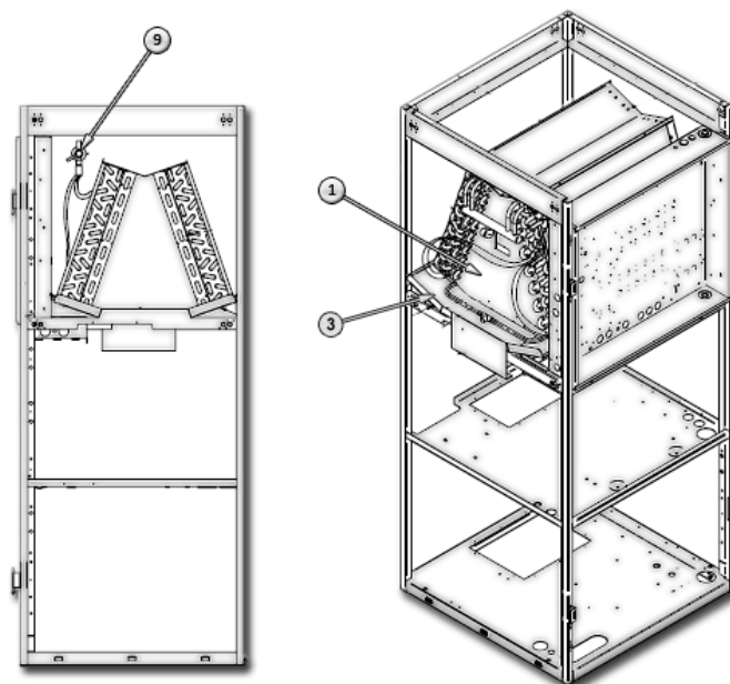
COIL OPTION DOWNFLOW RIFLED
