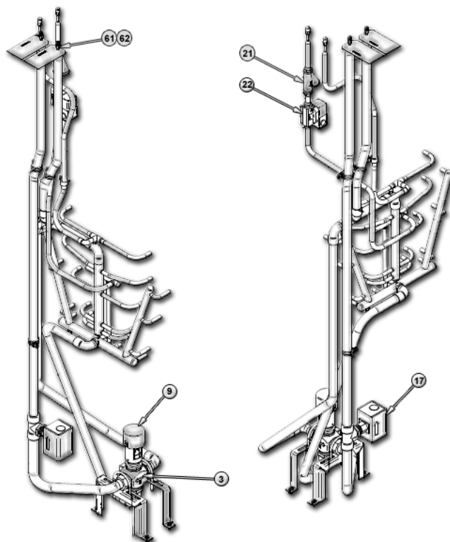
3-Way CW with FS w / HWRH
