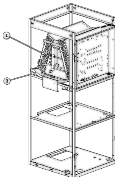
COIL OPTION CHILLED WATER DOWNFLOW
