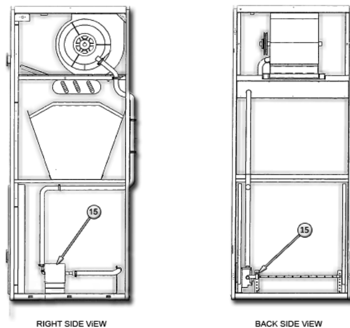
UPFLOW REAR RETURN
