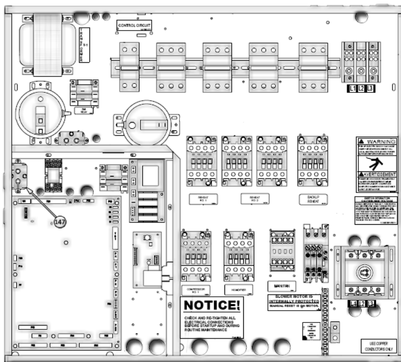
EP FAN COIL CIRCUIT BREAKER
