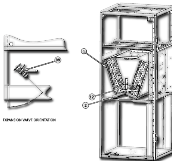
COIL OPTION 5T UPFLOW RIFLED
