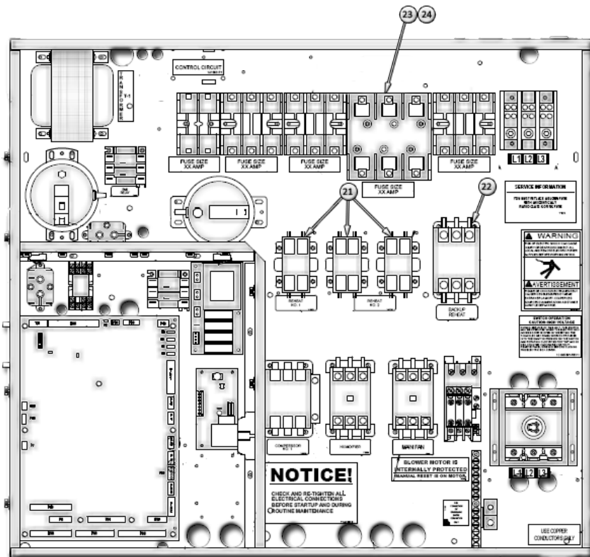
EP REHEAT FUSED
