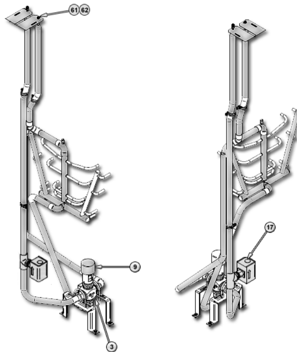
3-Way CW with FS
