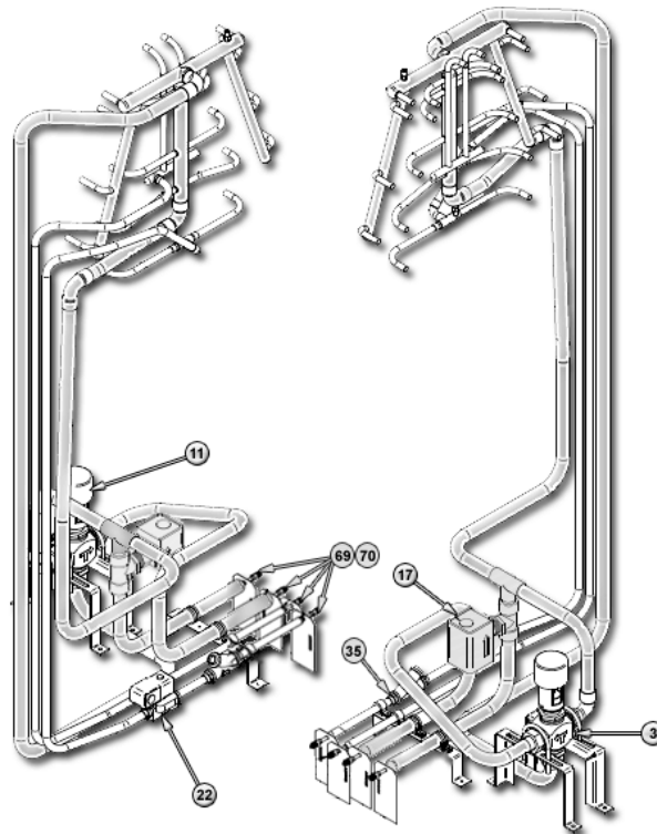
3-Way CW with FS w / HWRH
