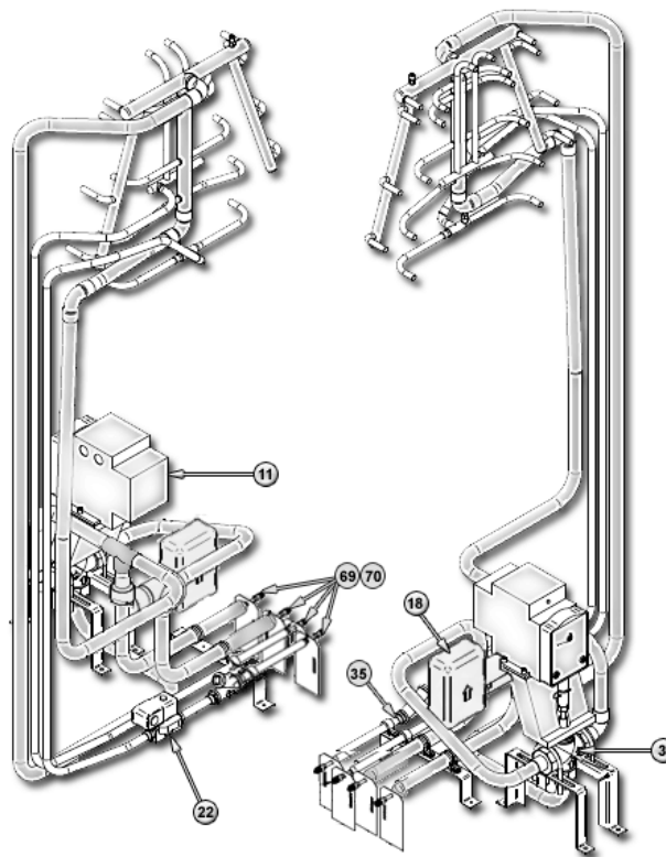
3-Way CW HP with FS w/HWRH
