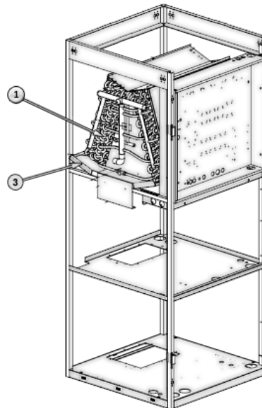
COIL OPTION 5T CHILLED WATER DOWNFLOW
