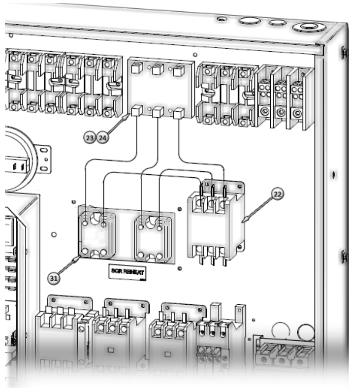
EP OPTION WITH SCR REHEAT
