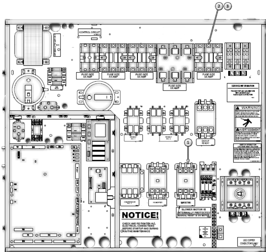
EP MOTOR CIRCUIT FUSED
