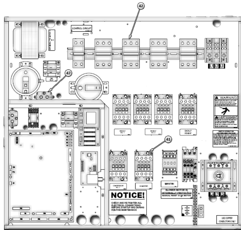
EP HUMIDIFIER CIRCUIT BREAKER
